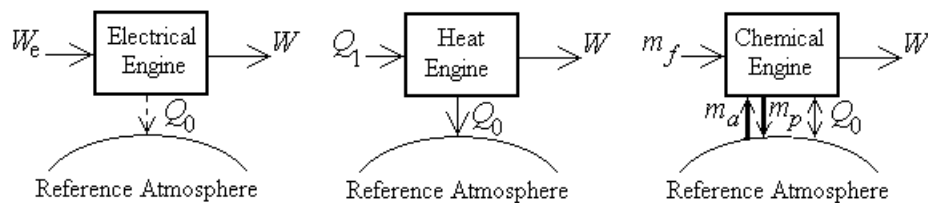
Fig. 3.2. Sketch of the different types of engines from a thermodynamics point-of-view: work engine (here represented by an electrical motor), heat engine, and chemical engine fed by a mass of fuel (and a mass of ambient air).
