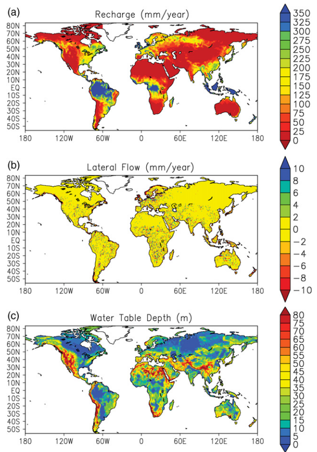
Figure 2. (a) Recharge ( \text{mm y}^{-1} ) and modeled (b) lateral flow ( \text{mm y}^{-1} ) and (c) water table depth (m). Values are shown averaged to 1^\circ resolution.
