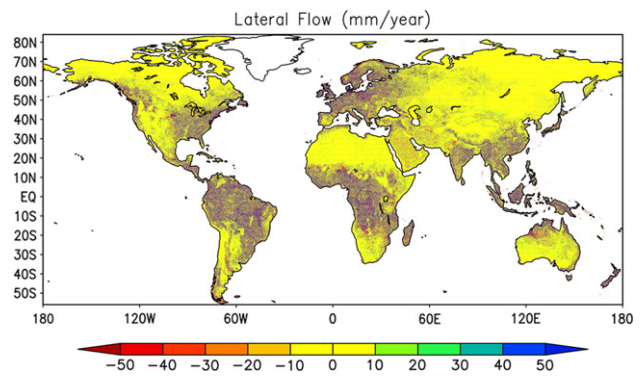
Figure 3. Modeled lateral flow ( \text{mm y}^{-1} ). Values are shown averaged to 0.1^\circ resolution.
