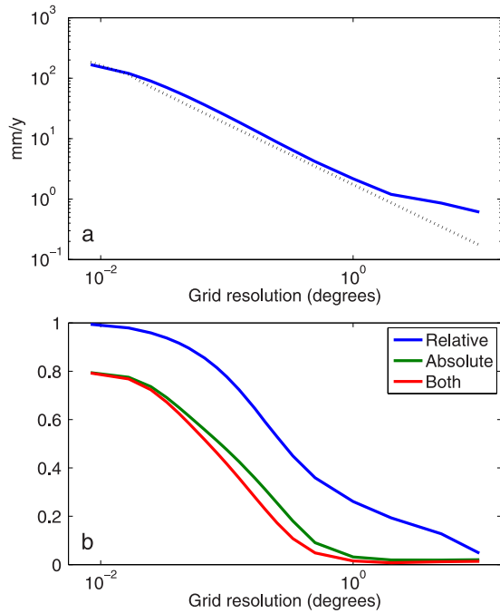
Figure 1. (a) Global mean groundwater lateral flow magnitude |L| as a function of grid spacing (solid line). The dashed line shows the relationship expected for large grid spacing from equation (5) with R = 107 \text{ mm y}^{-1} , f = 0.144 , and s = 30'' . (b) Area fraction of grid cells with substantial groundwater lateral flow magnitude |L| as a function of grid spacing. The fractions shown are for a relative magnitude criterion ( |L| > 0.1R ), an absolute magnitude criterion ( |L| > 10 \text{ mm y}^{-1} ), and for a combined threshold requiring both criteria.
