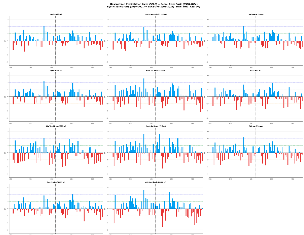
Figure 8. Standardised Precipitation Index at the medium-term scale (SPI-6) for the eleven stations of the Sebou basin (1980–2024), ordered by ascending altitude. Blue bars indicate wet periods ( \text{SPI-6} \geq 0 ) and red bars indicate dry periods ( \text{SPI-6} < 0 ). Blue bars indicate wet periods ( \text{SPI} \geq 0 ) and red bars indicate dry periods ( \text{SPI} < 0 ). The vertical dashed line marks the transition between the OBS (1980–2001) and bias-corrected ERA5-QM (2002–2024) series.
