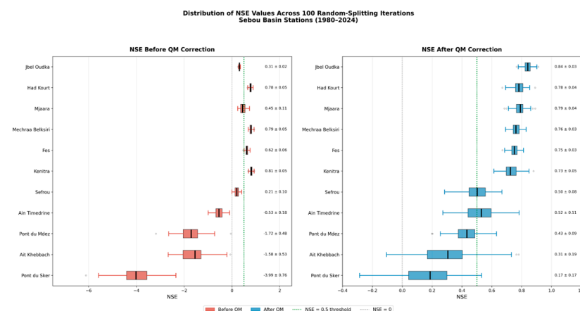
Figure 5. Distribution of NSE values across 100 random-splitting cross-validation iterations for the eleven stations of the Sebou basin. Boxes represent the interquartile range (Q25–Q75), the vertical line indicates the median, and whiskers extend to Q10 and Q90. The green dashed line indicates the NSE = 0.5 threshold.
