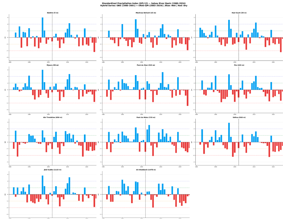
Figure 7. 12-month Standardised Precipitation Index (SPI-12) for the 11 stations of the Sebou basin (1980–2024). Blue bars indicate wet periods ( SPI \geq 0 ) and red bars indicate dry periods ( SPI < 0 ). The vertical dashed line marks the transition between the OBS (1980–2001) and bias-corrected ERA5-QM (2002–2024) series.
