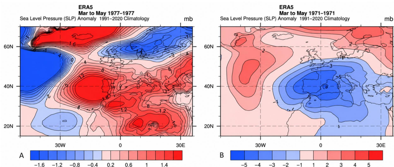
Figure 12. Anomalies of atmospheric pressure at sea level in spring during the positive phase of the EAP of the year 1977 ( A ) and the negative phase of the EAP of the year 1971 ( B ) (Data source: https://psl.noaa.gov/data/getpage/ , accessed on 26 10 2026).
