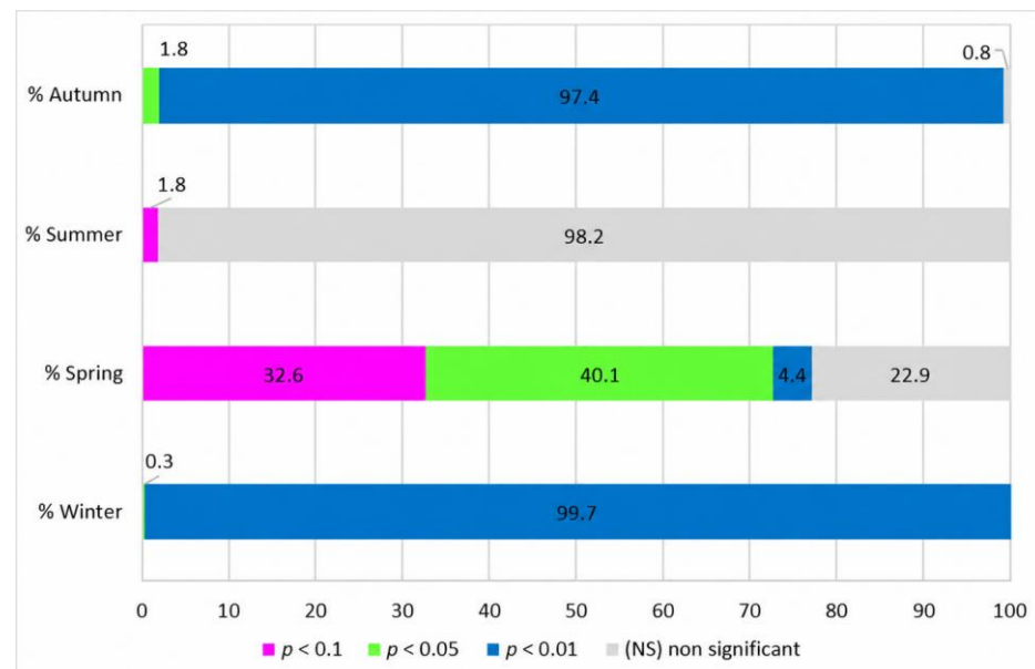
Figure 2. Percentage of grid points having a significant correlation between seasonal rainfall and NAO at thresholds 0.1, 0.05 and 0.01 (NS: non-significant correlation).
