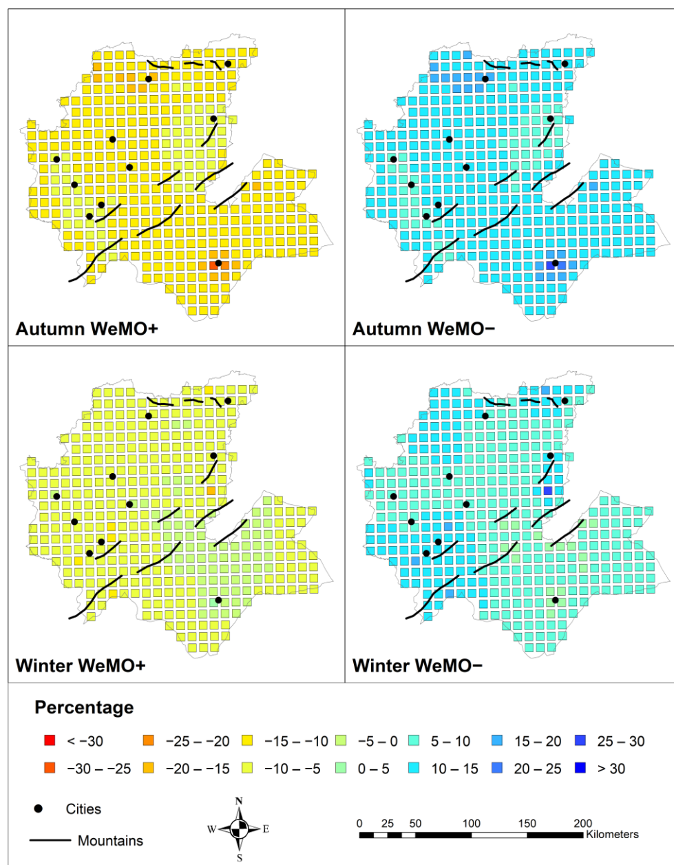
Figure 16. Percentage (%) of change in average autumn and winter precipitation according to the WeMO + and WeMO − phases..
