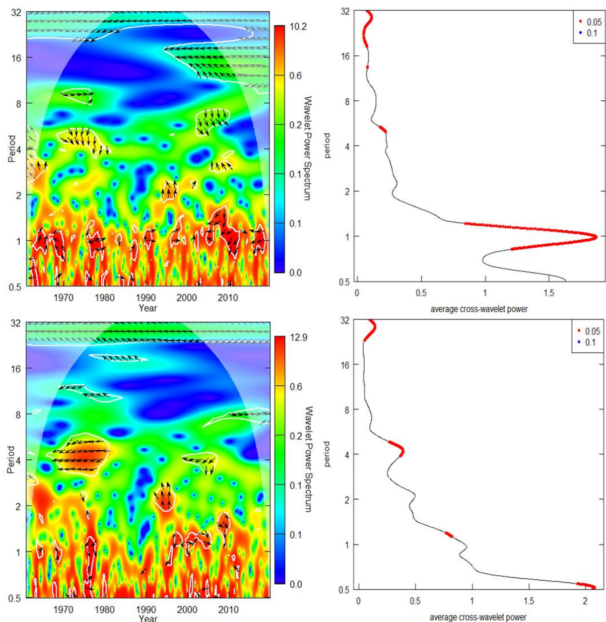
Figure 19. Wavelet coherence analysis between the EAP index and monthly precipitation at Aknoul (top) and Outat El Haj (bottom). Arrows pointing to the right indicate a positive correlation; those
