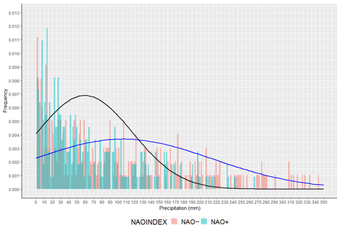
Figure 4. Histogram and smoothed probability density function for monthly rainfall data from the Ifrane station according to the two phases of the NAO index (the blue line NAO−, the black line NAO+).
