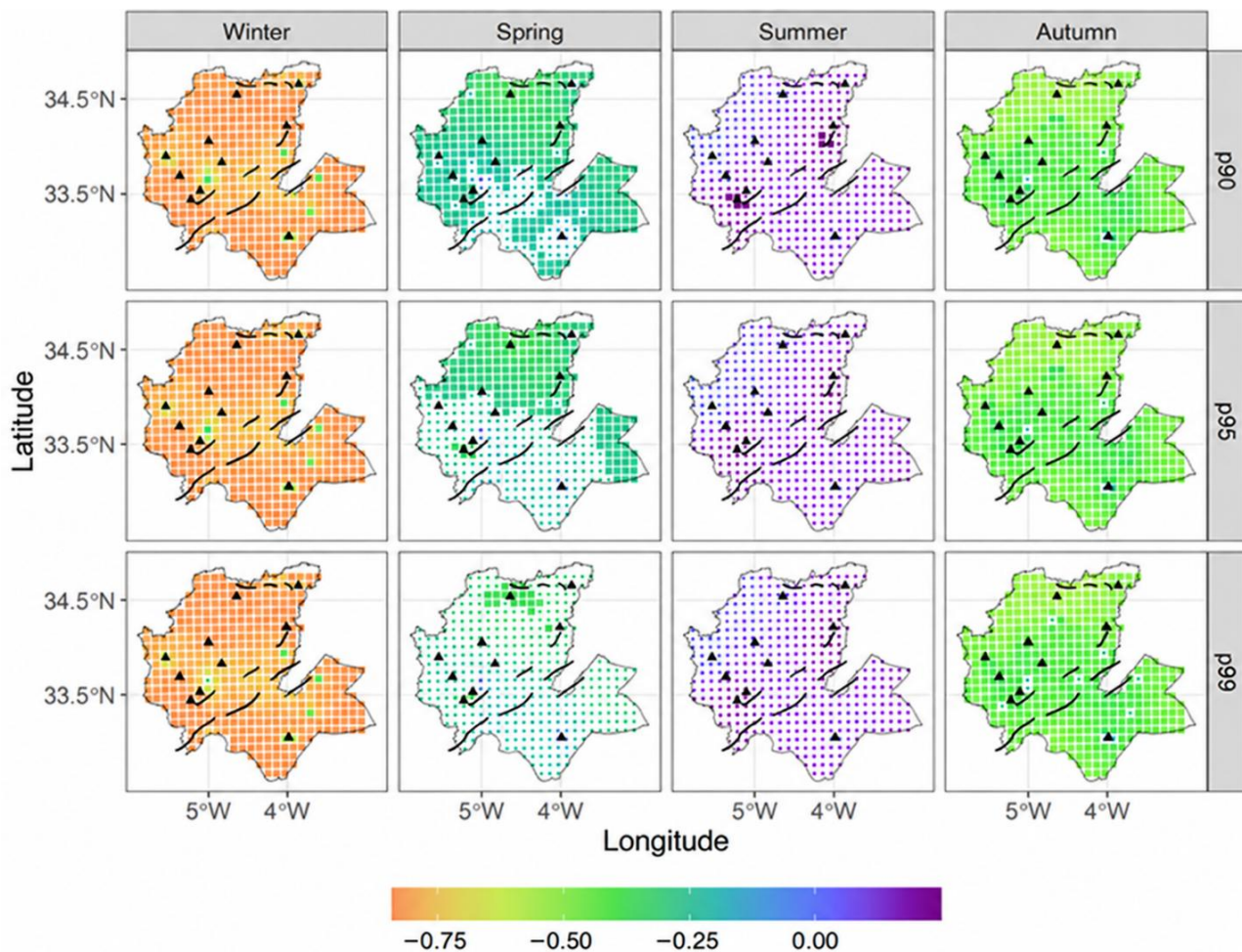
Figure 3. Correlation coefficient by grid points between rainfall and NAO of the four seasons (Square dimensions indicate the significance level of the correlations: large squares: significant correlation, small squares otherwise; colors show values of CC).
