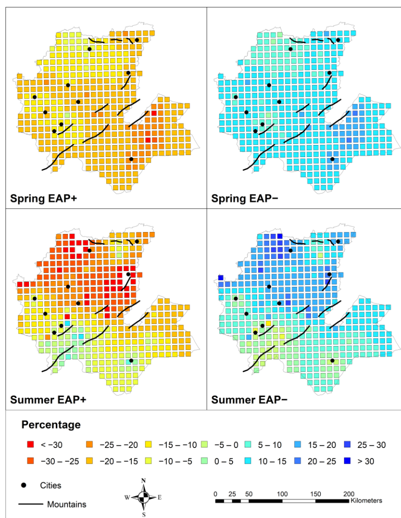
Figure 11. Percentage (%) of change in average spring and summer precipitation according to the EAP+ and EAP- index.
