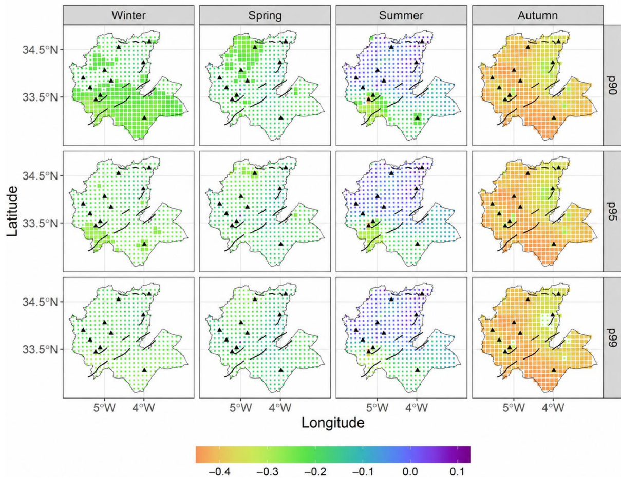
Figure 14. Correlation coefficient between seasonal rainfall and the WeMO index at each grid point. Colors indicate the values of the Pearson correlation coefficient, while square size indicates statistical significance: large squares denote significant correlations and small squares denote non-significant correlations.
