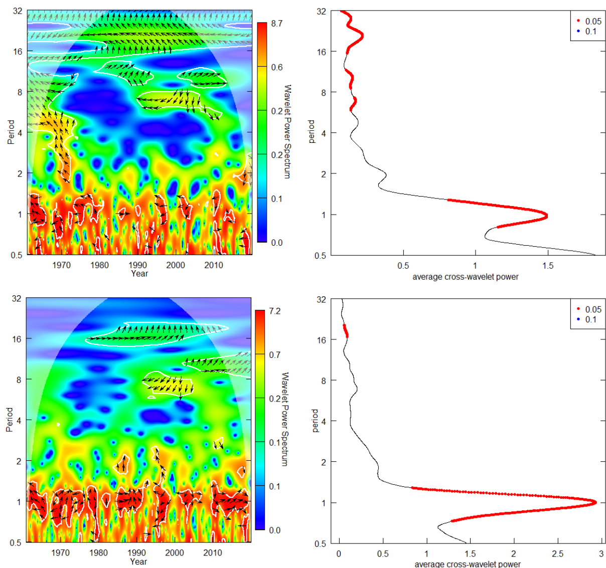
Figure 20. Wavelet coherence analysis between the WeMO index and monthly precipitation at Aguelman Sidi Ali ( top ) and Tafrant ( bottom ). Arrows pointing to the right indicate a positive correlation, those pointing to the left indicate a negative correlation, and areas enclosed in white lines indicate statistically significant correlation. The right-hand panels show the time-averaged cross-wavelet power as a function of period. The black curve represents the average cross-wavelet power; red markers indicate periods significant at the p < 0.05 level.
