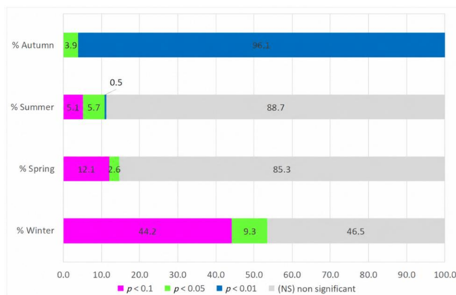
Figure 13. Percentage of grid points with a significant correlation between seasonal rainfall and WeMO oscillation at thresholds 0.1, 0.05 and 0.01 (NS: non-significant correlation).
