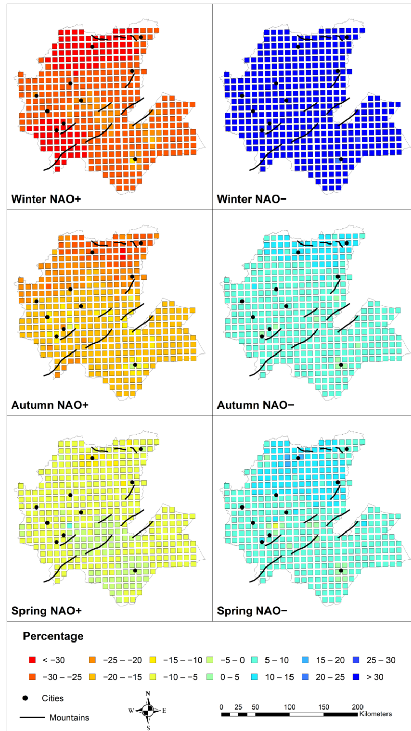
Figure 5. Percentage increase or reduction in precipitation relative to the long-term average according to the two phases of the NAO index for winter, autumn and spring.
