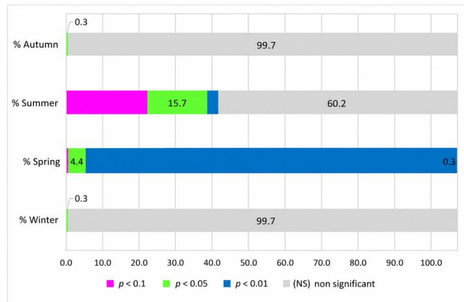
Figure 7. Percentage of grid points with a significant correlation between seasonal rainfall and EA oscillation at thresholds 0.1, 0.05 and 0.01 (NS: non-significant correlation).
