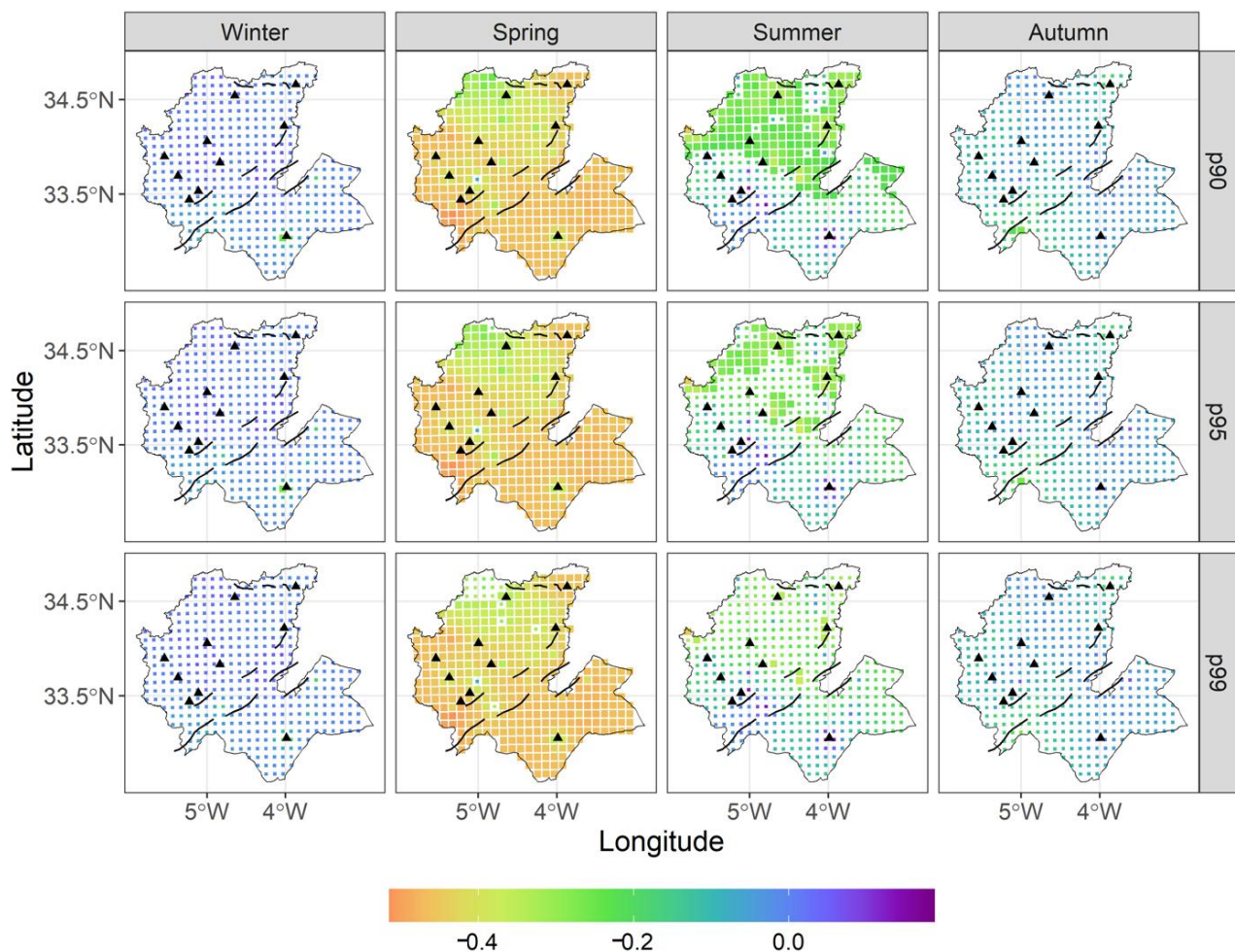
Figure 8. The correlation coefficient between rainfall of the four seasons and EAP index. (Square dimensions indicate the significance of the correlations: large squares: significant correlation, small squares otherwise).
