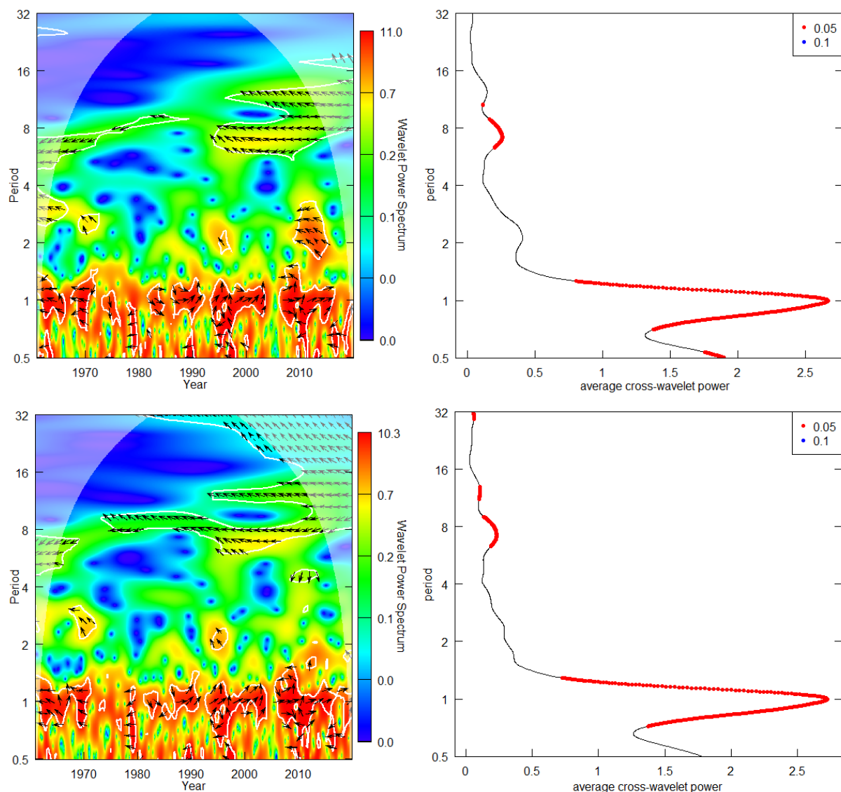
Figure 18. Wavelet coherence analysis between the NAO index and monthly precipitation at the Bab Ounder ( top ) and Tissa ( bottom ). Arrows pointing to the right indicate a positive correlation, those pointing to the left indicate a negative correlation, and areas enclosed in white lines indicate statistically significant correlation. The right-hand panels show the time-averaged cross-wavelet power as a function of period. The black curve represents the average cross-wavelet power; red markers indicate periods significant at the p < 0.05 level.
