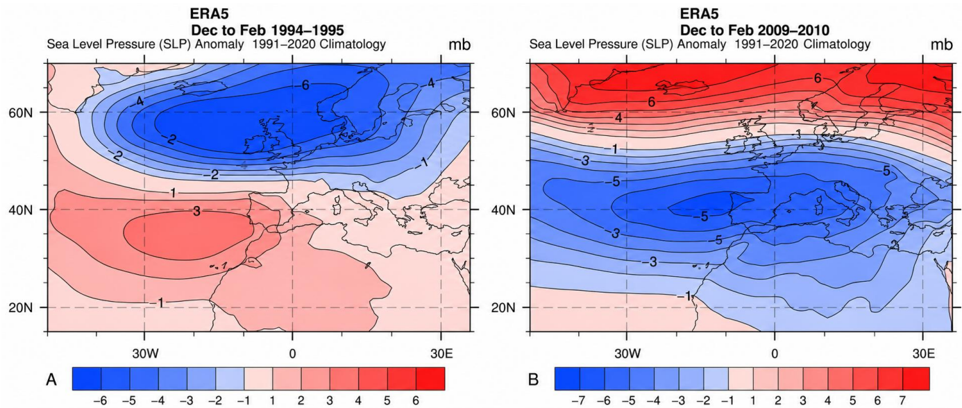
Figure 6. Anomalies of atmospheric pressure at sea level in winter during a positive phase of the NAO in the winter of 1994–1995 (A) and a negative phase of the NAO in the winter of 2009–2010 (B) (Data source: https://psl.noaa.gov/data/getpage/ , accessed on 26 October 2026).
