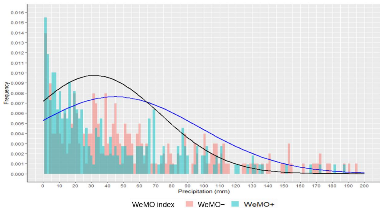
Figure 15. Histogram and smoothed PDF for monthly rainfall data from the Ain Aïcha station according to the two phases of the WeMO index (the blue line WeMO−, the black line WeMO+).
