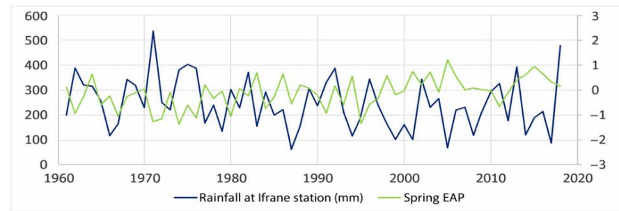
Figure 9. Interannual variability of spring rainfall at Ifrane station and the EAP index of the same season during the period 1961–2019. (The negative correlation between the two series is significant at the threshold \alpha = 0.01 ).
