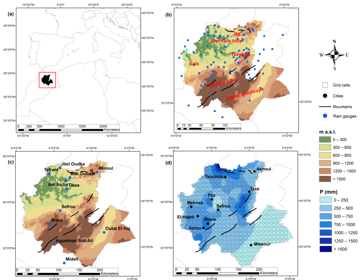
Figure 1. (a) localization of the study area (red box); (b) topography and rain gauge stations; (c) topography and rain gauge stations used for the wavelet analysis; (d) grid points, interpolated precipitation, and main cities. Black lines in (b–d) represent the main ridges of mountains.
