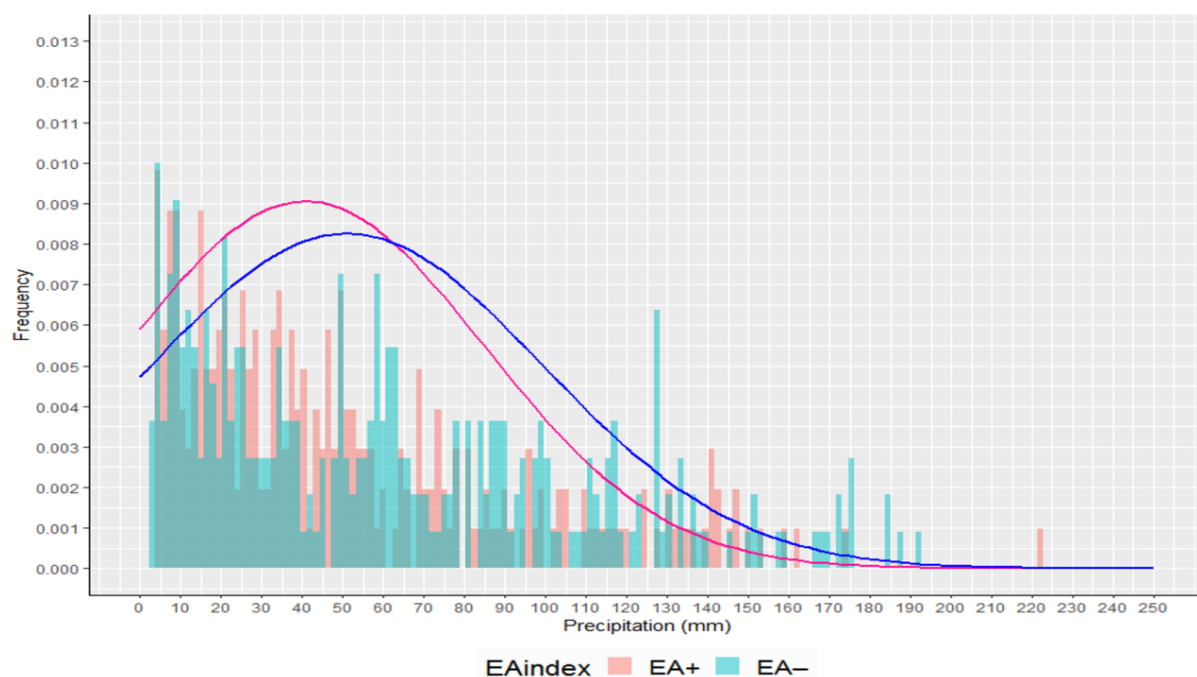
Figure 10. Histogram and smoothed probability density function for monthly rainfall data from the Sefrou station (S65) according to the two phases of the EAP index (the blue line EAP−, the pink line EAP+).
