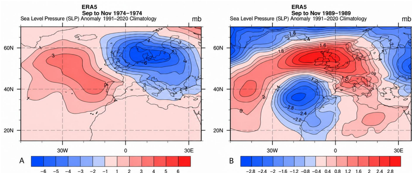
Figure 17. Anomalies of atmospheric pressure at sea level in autumn during the positive WeMO phase of the year 1974 (A) and the negative WeMO phase of the year 1989 (B) (Data source: https://psl.noaa.gov/data/getpage/ , accessed on 26 10 2026).
